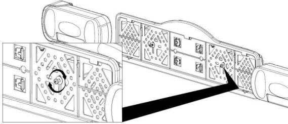
Figure 5: Mounting the license plate holder
